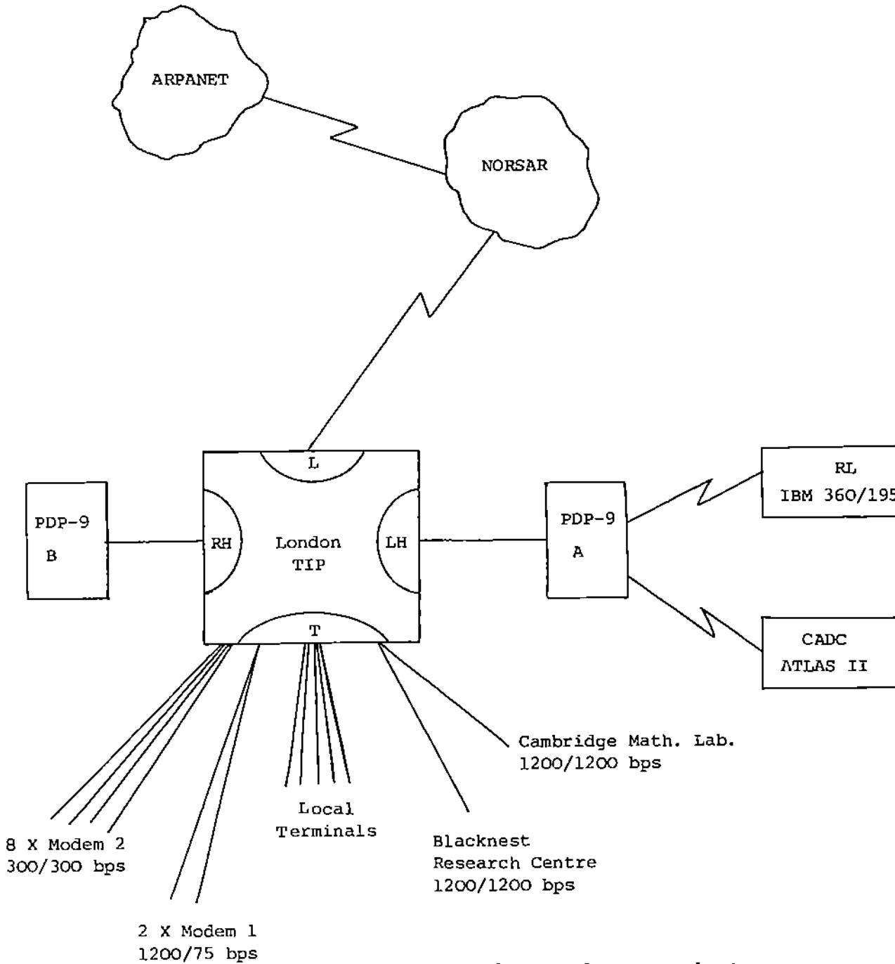
Figure 1. Schematic of UCL configuration, July 1975.
