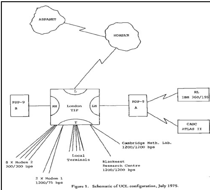
Figure 1. Schematic of UCL configuration, July 1975.
